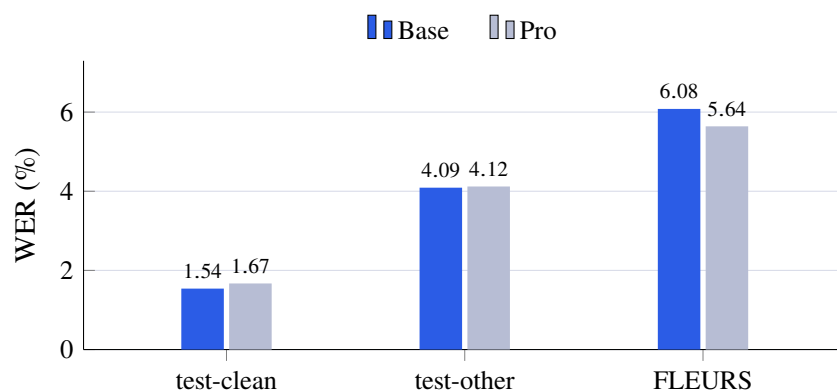
Figure 1: Word error rate, Base and Pro on the same seeded samples (Table 1, right-hand columns).
